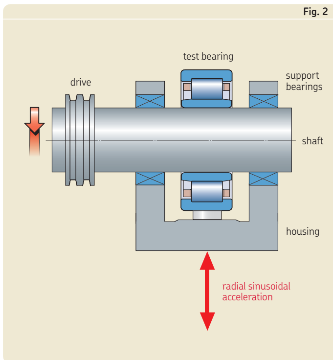
Principle of test rig for dynamic cage strength testing
